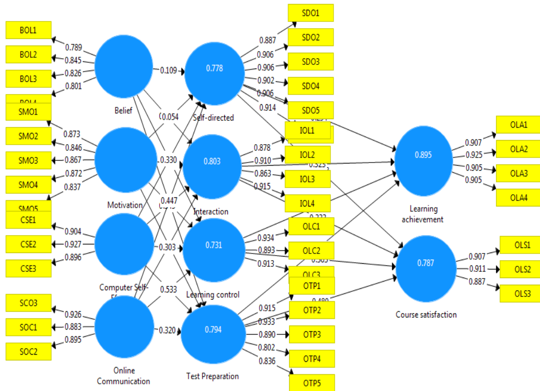
Figure 2. Data Analysis of Smart PLS-SEM All items loading >0.7 (very good)
